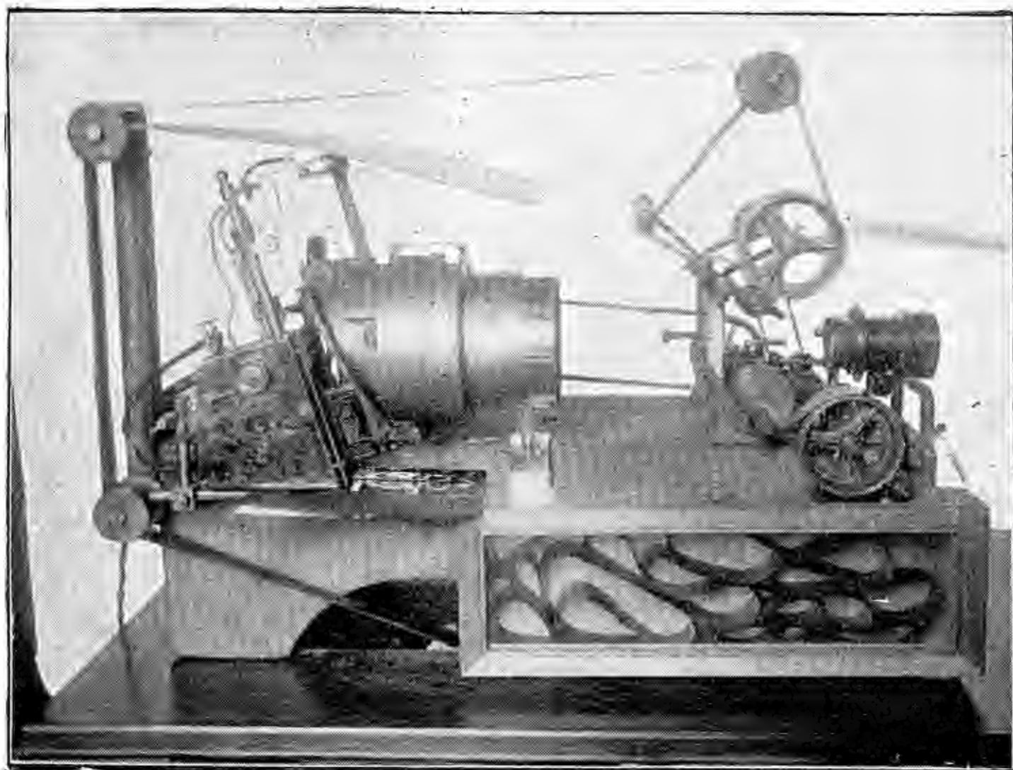
A LATER FORM JENKINS PROJECTING PHANTOSCOPE.
